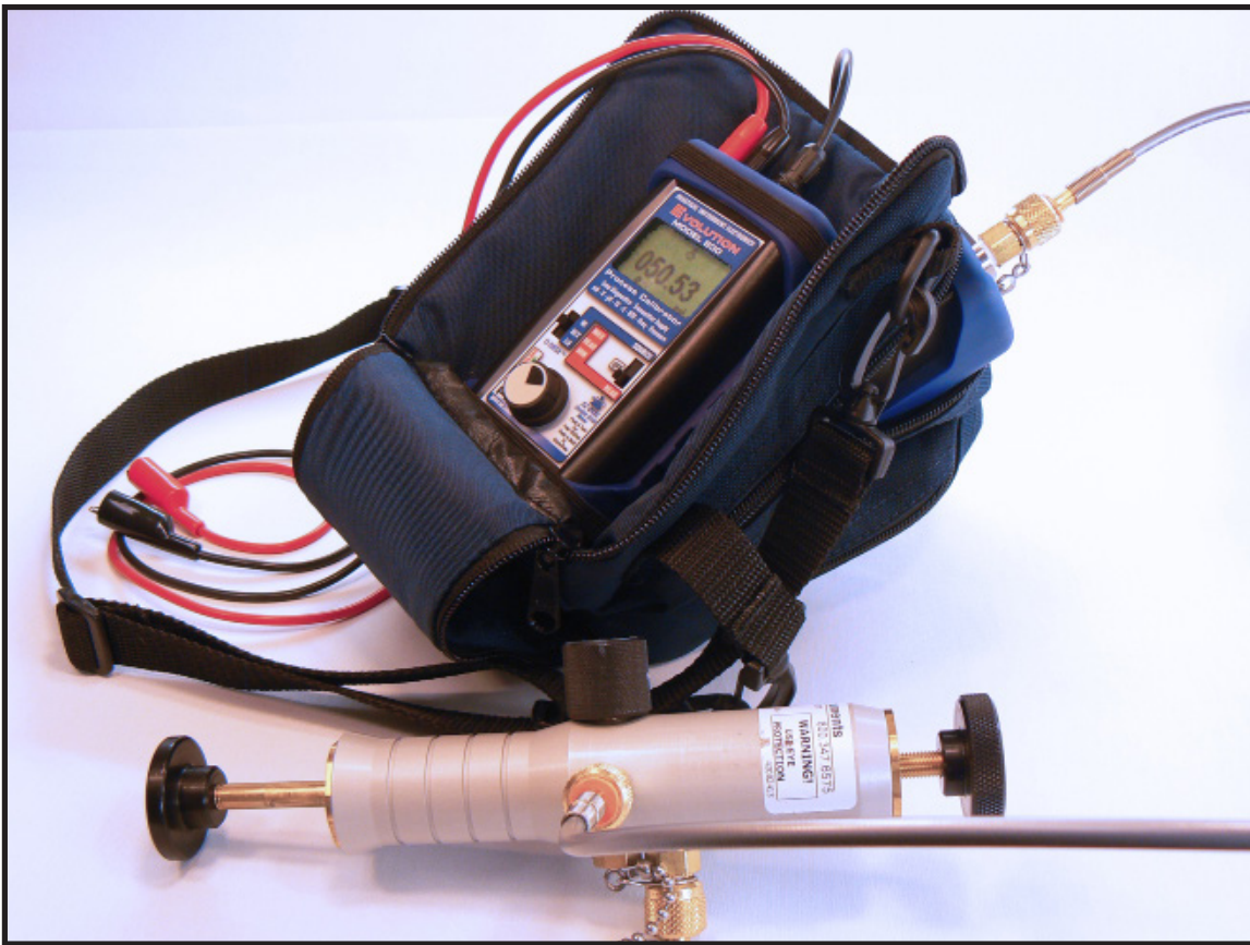
Hands free carrying case with pockets for the PIE 830 and the Pressure Module. Back of case has zipped pocket for the manual, test leads, hoses & pressure fittings.
