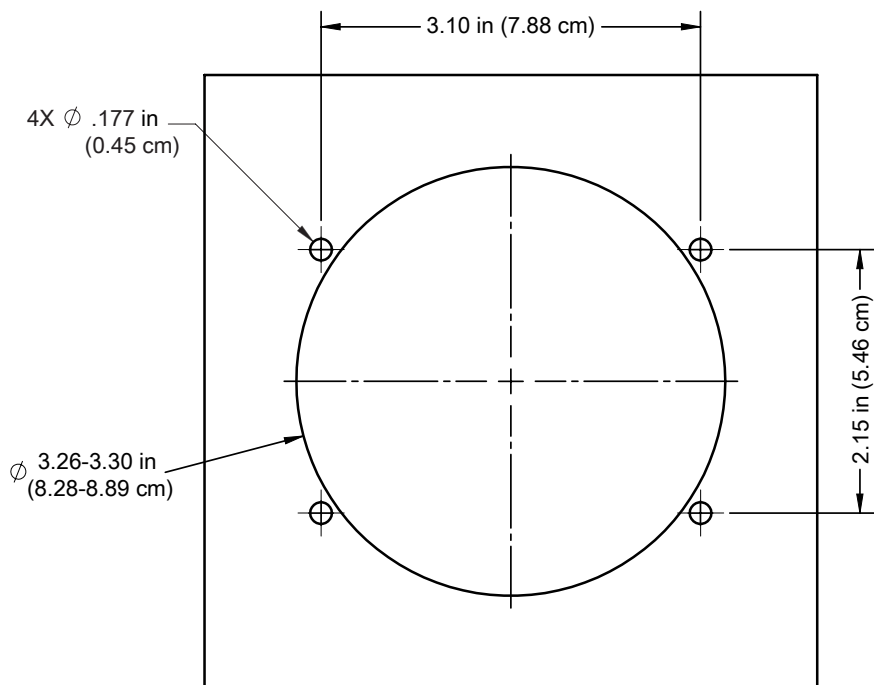
Diagram of Assembling Panel Mounting Kit
